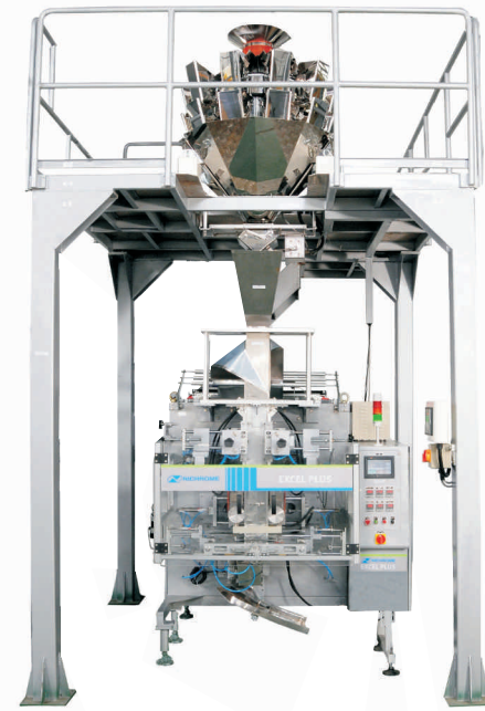
Excel Plus Multi-Head Weigher
